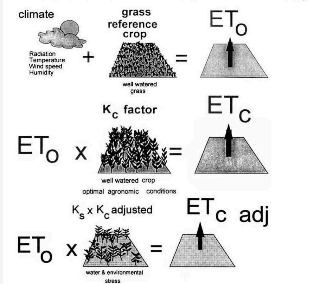
4. Reference ( ET_0 ), crop evapotranspiration under standard ( ET_c ) and non-standard conditions ( ET_{c\ adj} )
