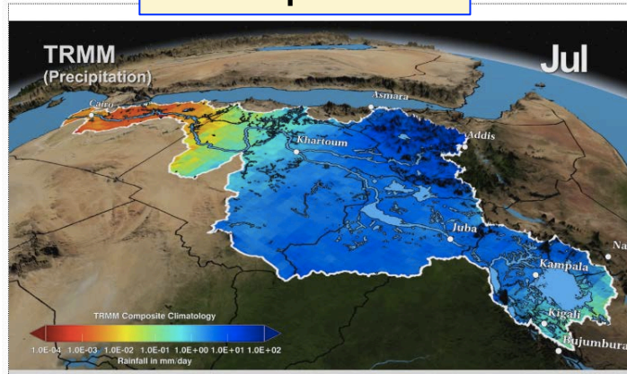
Precipitation
