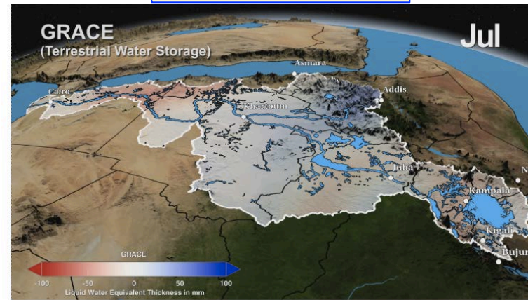
Terrestrial Water
