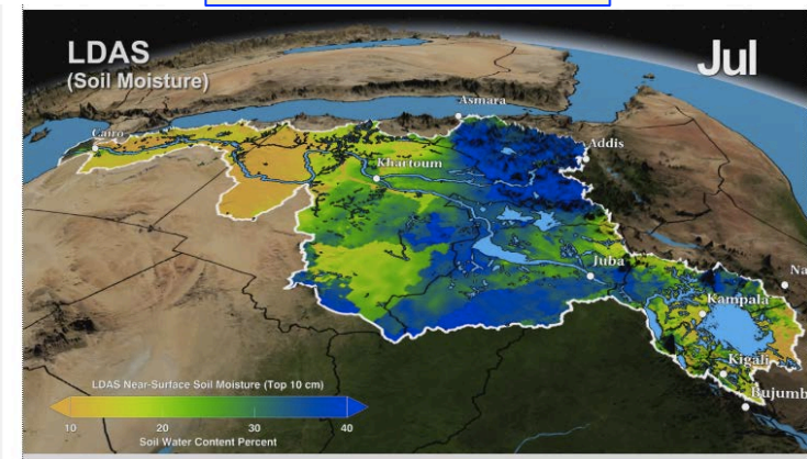
Soil Moisture
