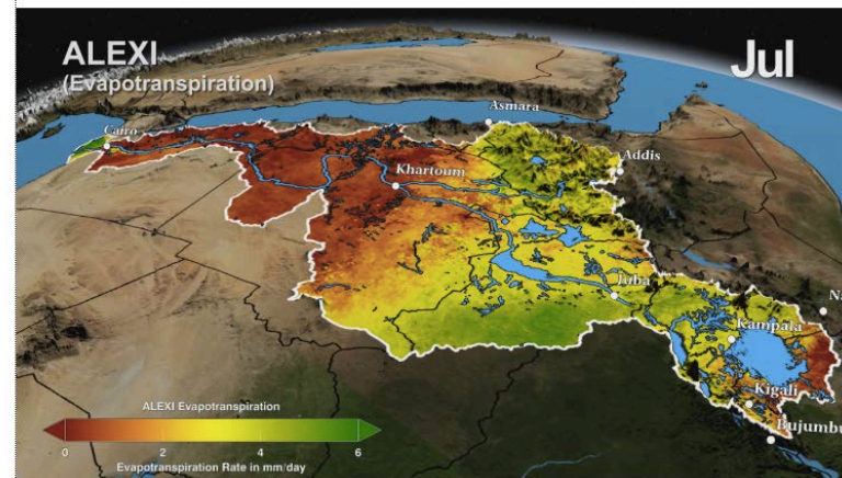
Evapotranspiration
